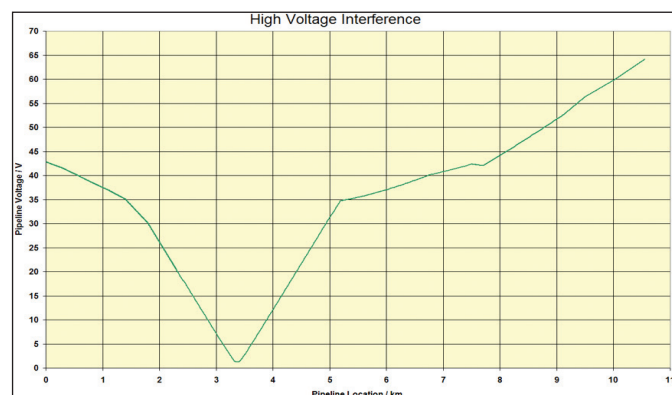
Calculation results caused by overhead line operating currents with earthing measures ( U_{\max} < 65 V according to German Standard)
